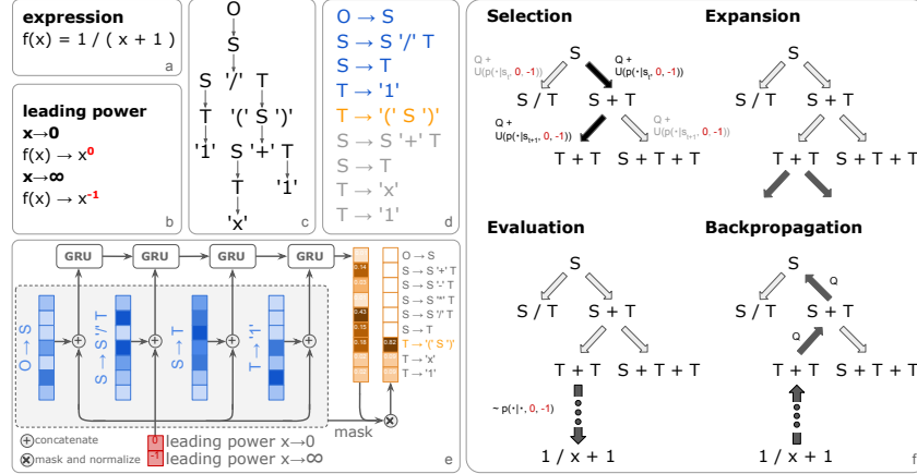
Figure 1: Model architecture. (a) Exemplary expression. (b) Leading powers of 1/(x+1) at 0 and \infty . (c) Parse tree of 1/(x+1) . (d) Production rule sequence, the preorder traversal of production rules in the parse tree. (e) Architecture of the model to predict the next production rule from the partial sequence. (f) Using the network in (e) conditioned on desired leading powers to guide MCTS.
