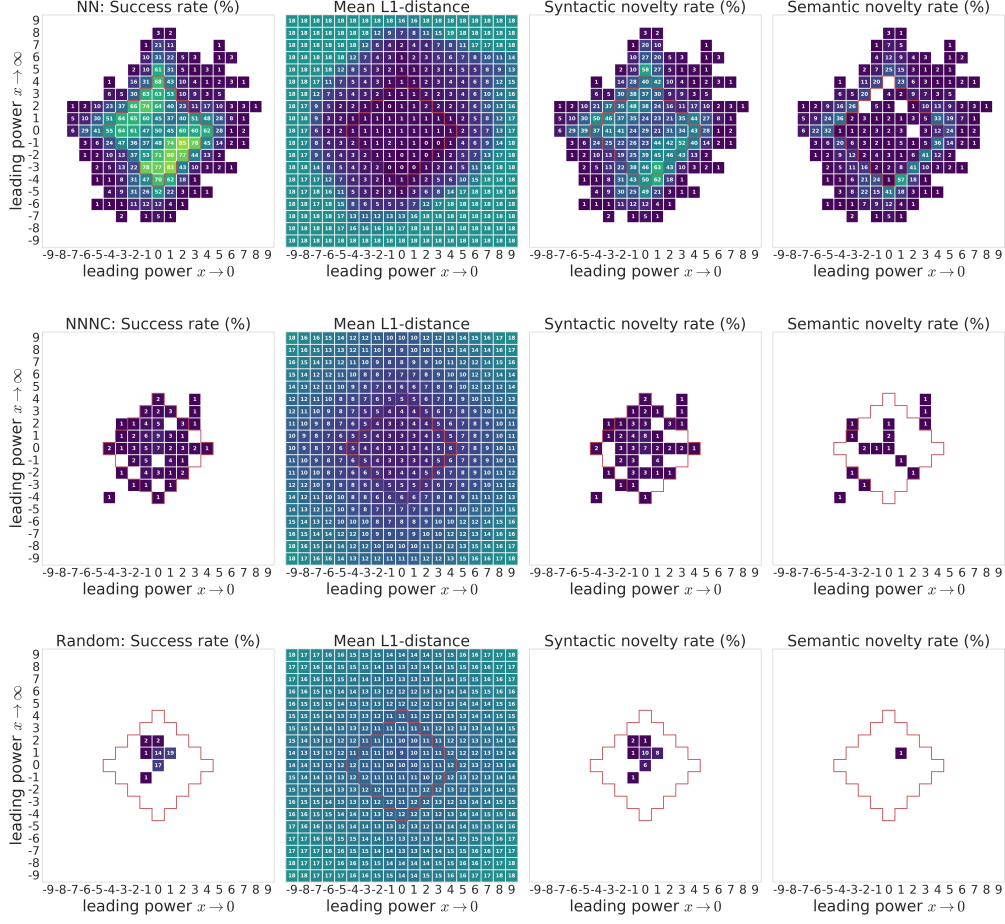
Figure E.1: Metrics for NN, NNNC and Random models on each condition within |P_{x \rightarrow 0}[f]| \leq 9 and |P_{x \rightarrow \inf}[f]| \leq 9 . Each column corresponds to a metric: success rate, mean L1-distance, syntactic novelty rate and semantic novelty rate, respectively. Conditions with M[f] \leq 4 are inside the red boundary. Conditions with zero success rate, syntactic novelty rate or semantic novelty rate are left blank in the corresponding plots.
