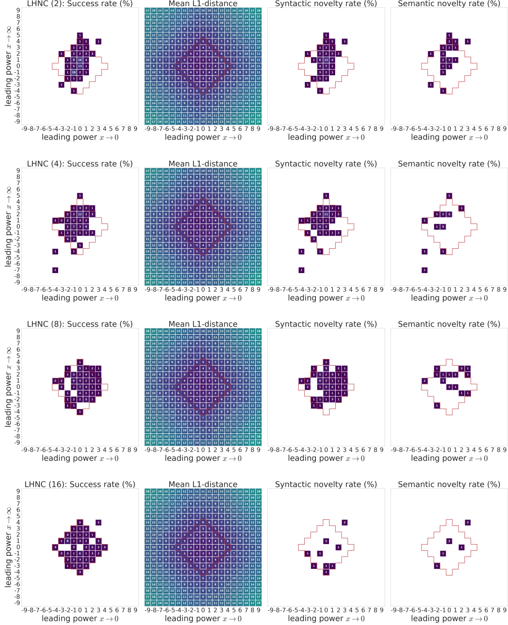
Figure E.4: Metrics for LHNC models with different history length on each condition within |P_{x \rightarrow 0}[f]| \leq 9 and |P_{x \rightarrow \inf}[f]| \leq 9 . Each column corresponds to a metric: success rate, mean L1-distance, syntactic novelty rate and semantic novelty rate, respectively. Conditions with M[f] \leq 4 are inside the red boundary. Conditions with zero success rate, syntactic novelty rate or semantic novelty rate are left blank in the corresponding plots.
