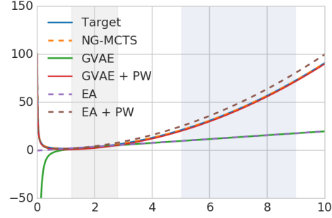
Figure 3: Plot of force field expressions found by each method. Grey area is the region to compute interpolation error \Delta g_{\text{int.}} and light blue area is the region to compute extrapolation error \Delta g_{\text{ext.}} .
