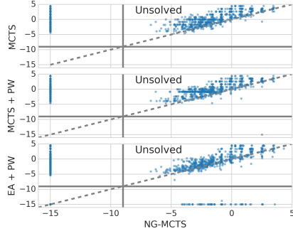
Figure 2: Extrapolation errors of symbolic regression methods in holdout set M[f] = 5 . Each expression is a point, where \log_{10} \Delta g_{\text{ext.}} obtained by NG-MCTS is on x-axis and those obtained by other three methods are on the y-axis.
