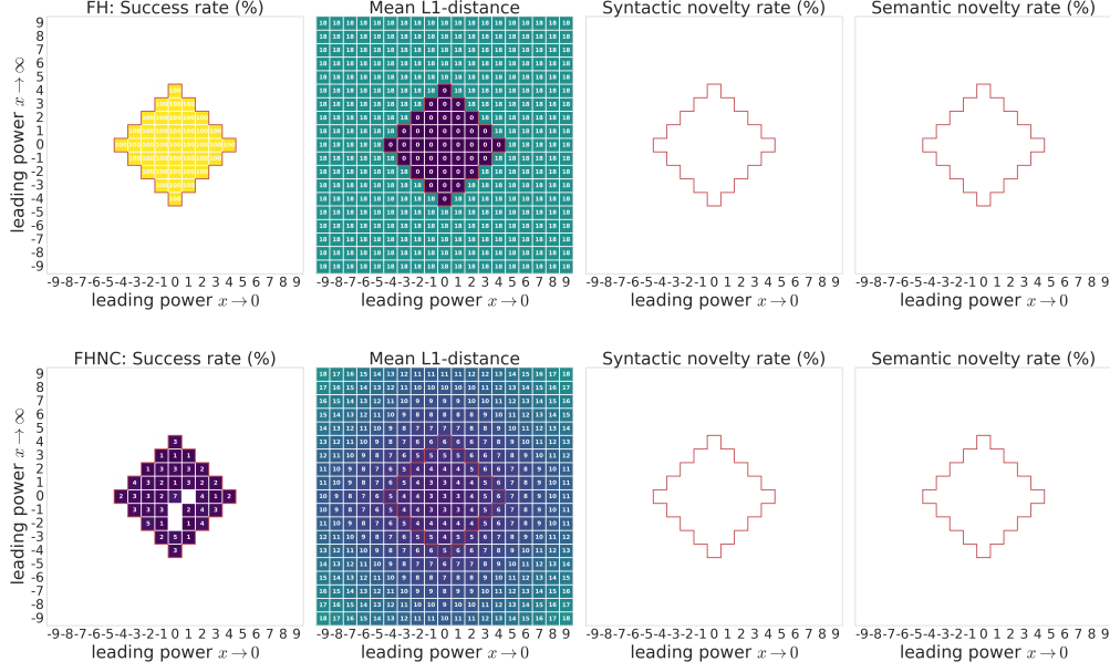
Figure E.2: Metrics for FH and FHNC models on each condition within |P_{x \rightarrow 0}[f]| \leq 9 and |P_{x \rightarrow \inf}[f]| \leq 9 . Each column corresponds to a metric: success rate, mean L1-distance, syntactic novelty rate and semantic novelty rate, respectively. Conditions with M[f] \leq 4 are inside the red boundary. Conditions with zero success rate, syntactic novelty rate or semantic novelty rate are left blank in the corresponding plots.
