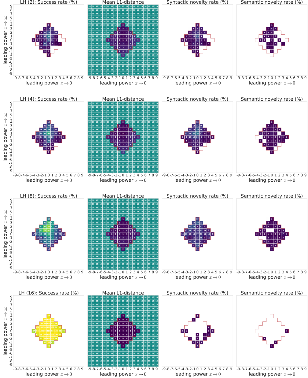
Figure E.3: Metrics for LH models with different history length on each condition within |P_{x \rightarrow 0}[f]| \leq 9 and |P_{x \rightarrow \inf}[f]| \leq 9 . Each column corresponds to a metric: success rate, mean L1-distance, syntactic novelty rate and semantic novelty rate, respectively. Conditions with M[f] \leq 4 are inside the red boundary. Conditions with zero success rate, syntactic novelty rate or semantic novelty rate are left blank in the corresponding plots.
