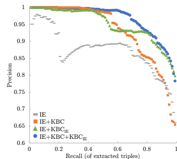
Figure 6: Precision Recall curves for NELL
