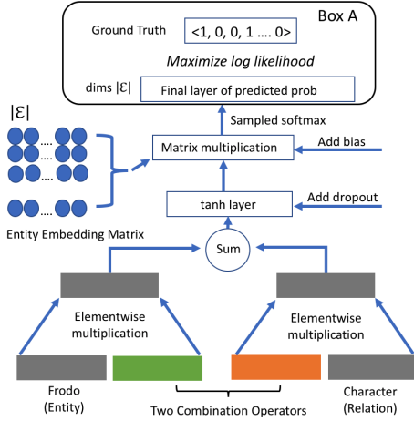
Figure 3: Base ProjE softmax architecture for KBC.
