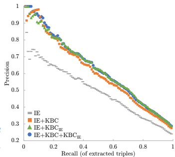
Figure 5: Precision Recall curves for NYT-FB
