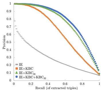
Figure 4: Precision Recall curves for CC-DBP
