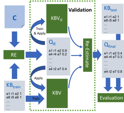
Figure 2: Pipeline for our RE solution.
